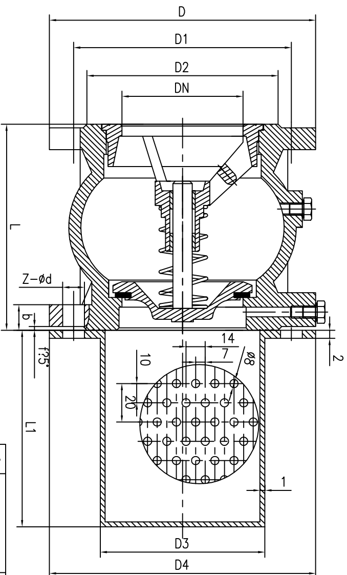
Flange Dimensions: BS EN1092-2
